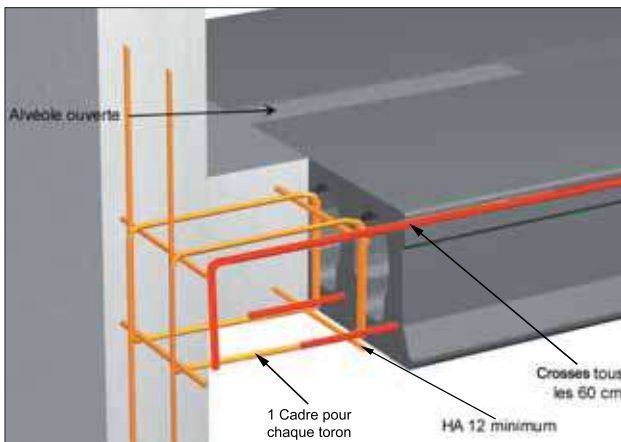
Console courte
